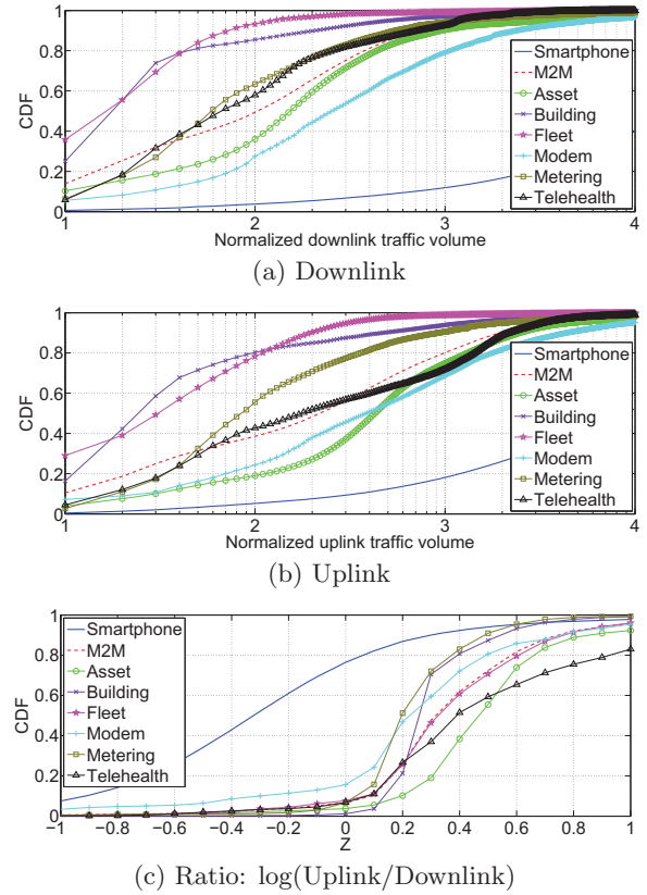
Figure 1: CDFs of aggregate downlink and uplink traffic volume.
