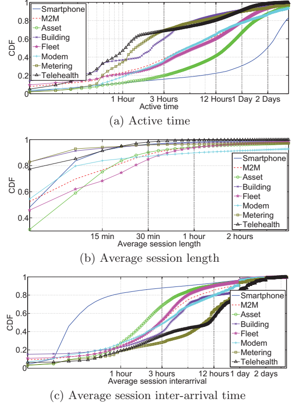
Figure 7: CDFs of active time, average session length, and session inter-arrival.
