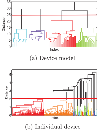
Figure 4: Dendrograms for hierarchical clustering.
