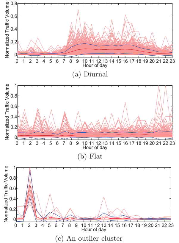
Figure 6: Cluster centroids identified using individual device traffic time series.
