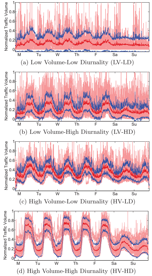
Figure 5: Cluster centroids identified using device models traffic time series.
