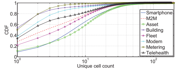
Figure 8: CDFs of unique cells for smartphone and M2M categories.
